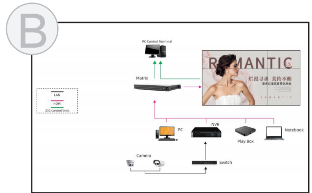
Matrix connection
