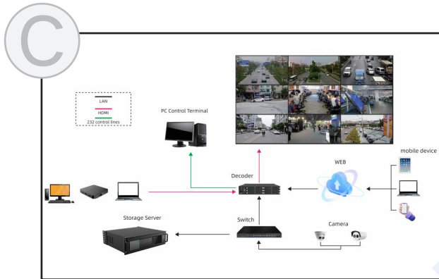
Decoder connection
